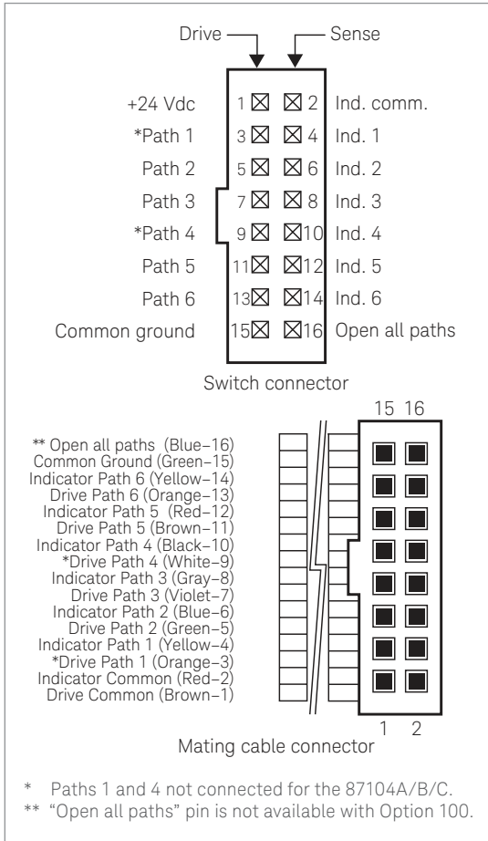
Figure 10. Drive connection diagrams with Option 161
