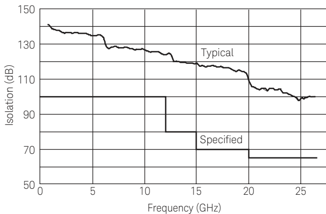
Figure 8. Isolation
