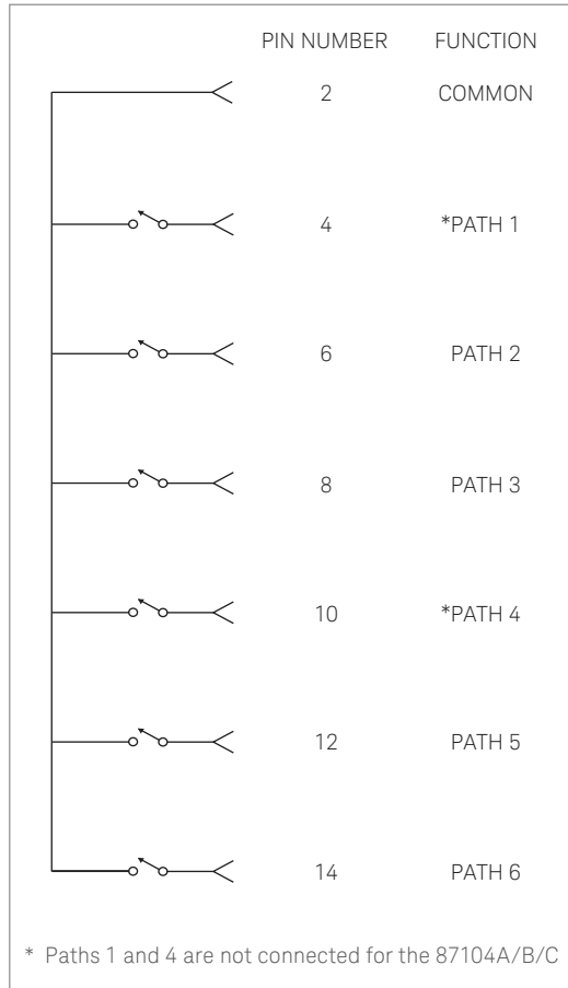
Figure 6. Pin function diagram
