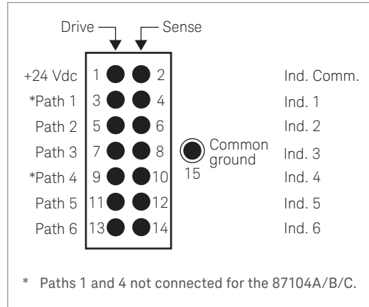
Figure 11. Drive connection diagrams with Option 100
