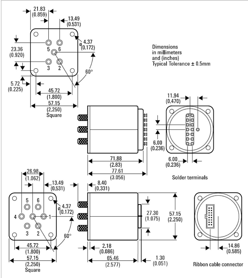
Figure 9. Product outlines
