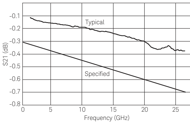
Figure 7. Insertion loss
